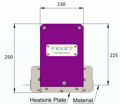
UV LAMP HEAD DIMENSIONS
