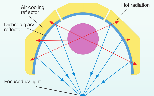
Highly Efficient Reflector Design
