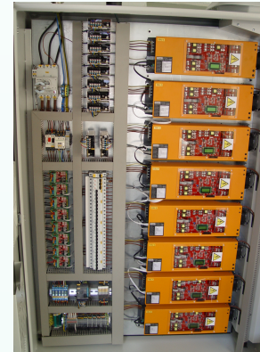
Main Electrical Cabinet
