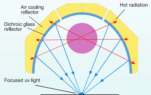
Highly Efficient Reflector Design
