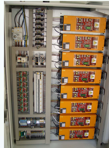
Main Electrical Cabinet
